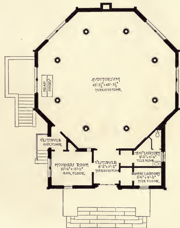
PLAN MENDESLESON MEMORIAL CHAPEL
